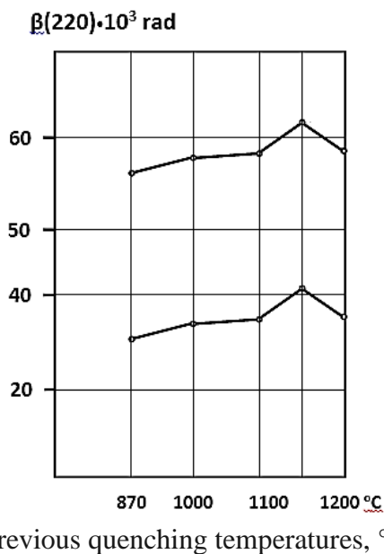
Fig. 1. Change in the parameters of the structure of steel U8A depending on the previous quenching and medium tempering.
